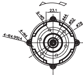
DIRECTION OF ROTATION
